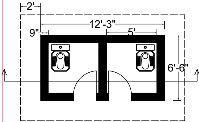
Plan View of toilet Block
