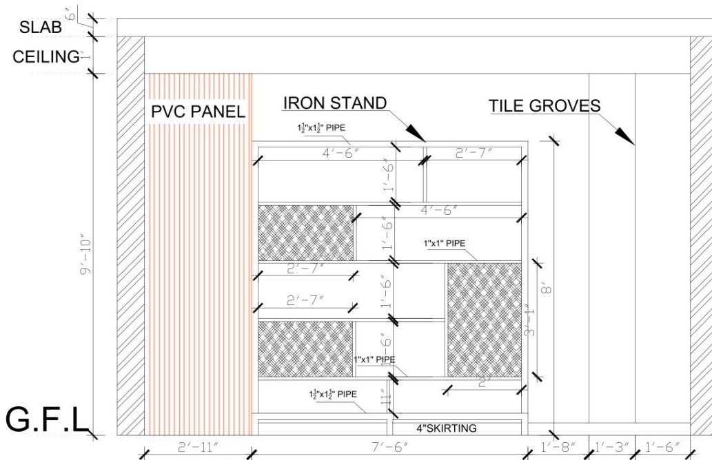
ELEVATION-4
