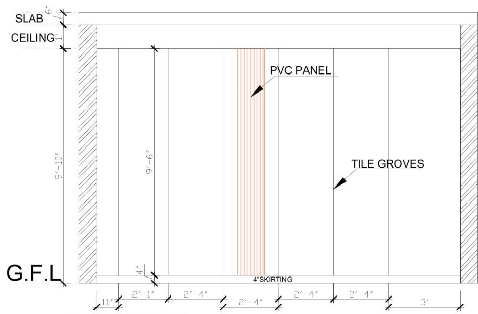
ELEVATION-4
